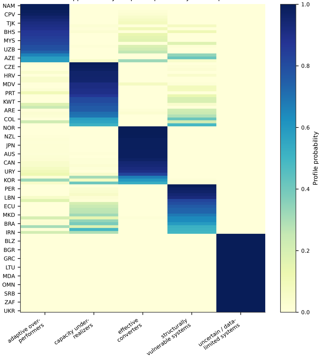
Supplementary full profile probability heatmap
