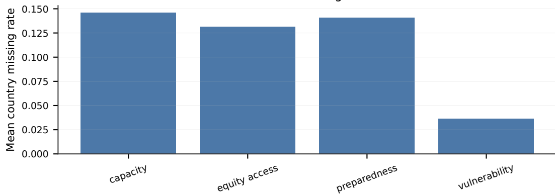
B. Indicators with highest missingness
