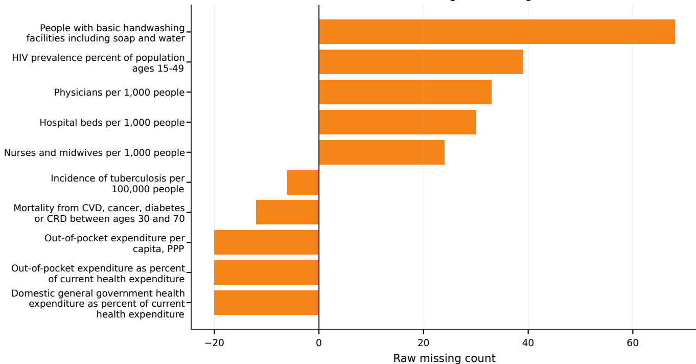
B. Indicators with highest missingness
