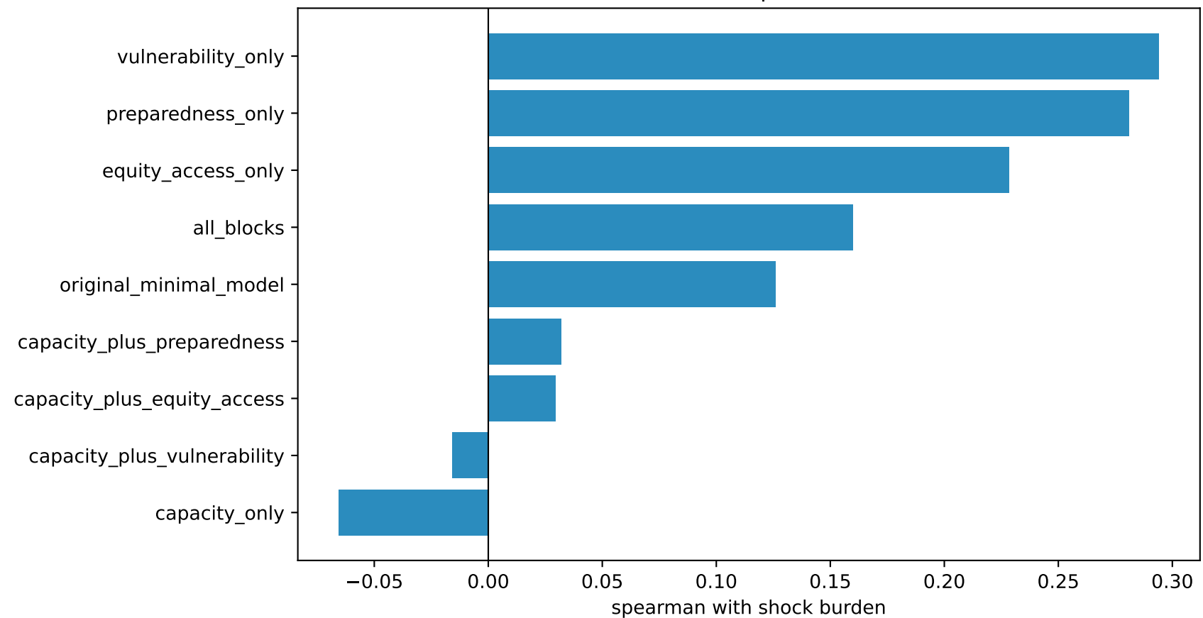
Block ablation performance
