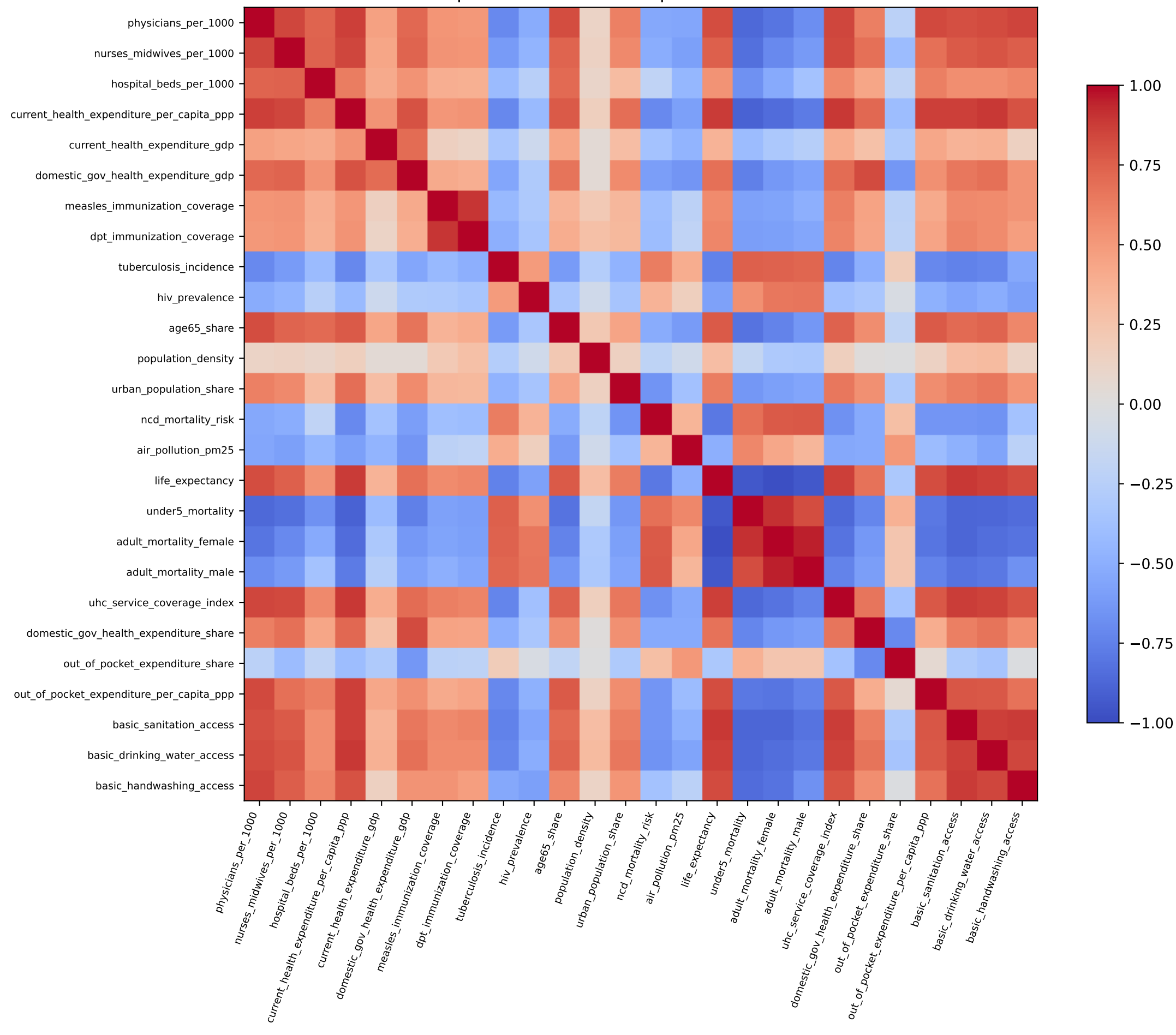
Expanded block feature Spearman correlations
