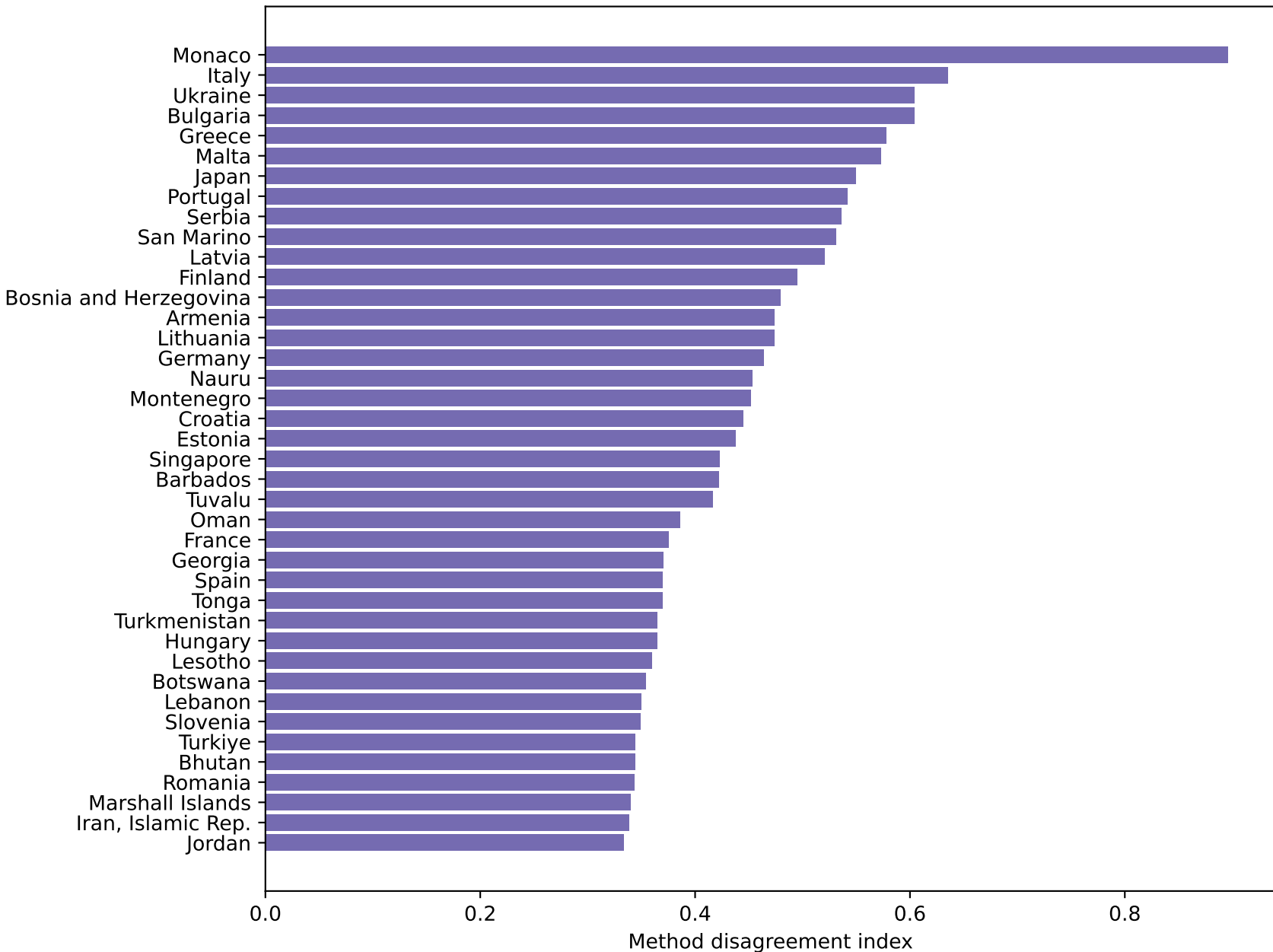
Most method-sensitive country ranks
