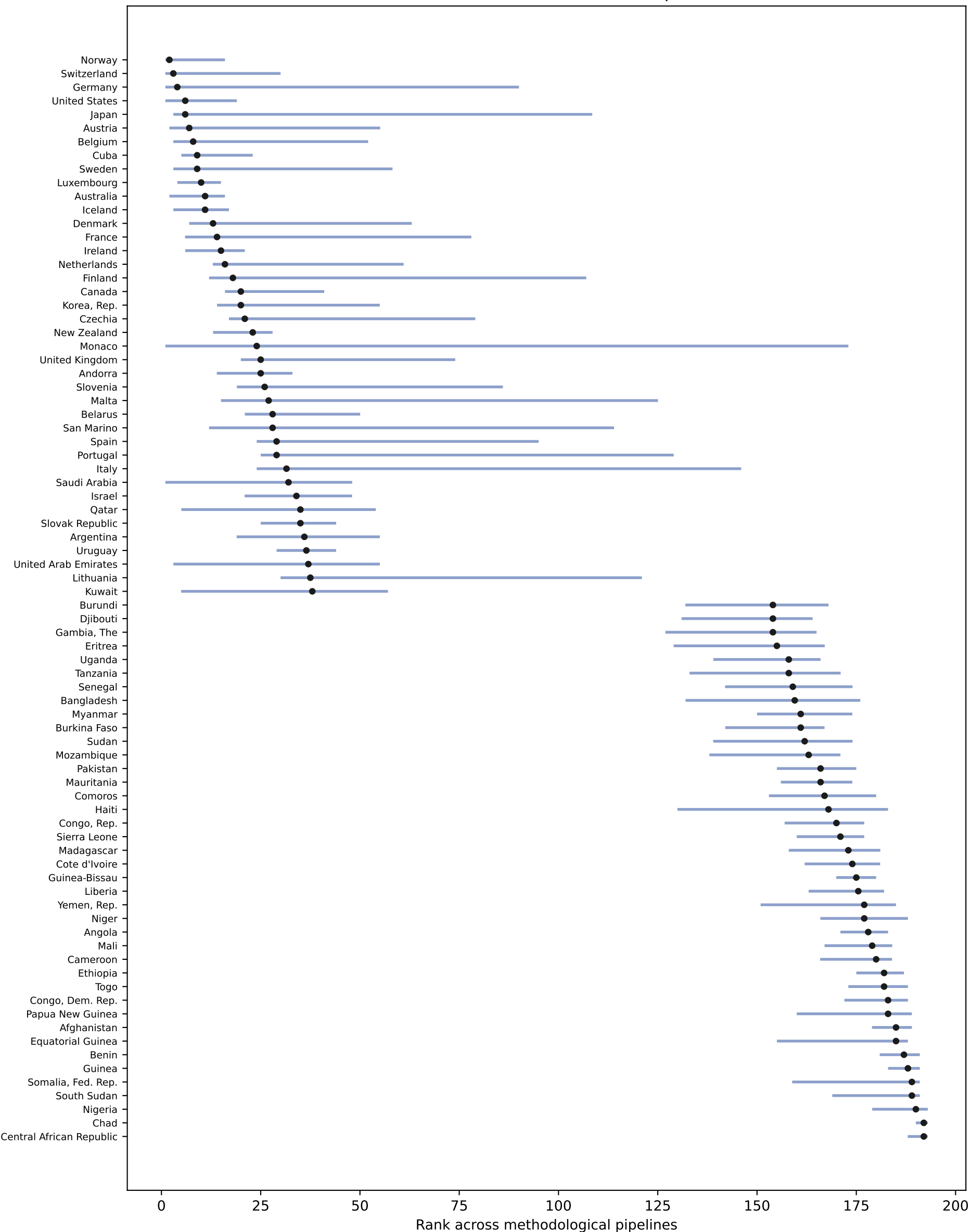
Consensus rank intervals, 5th to 95th percentile
