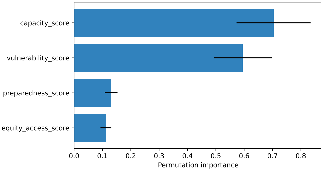
RF permutation importance
