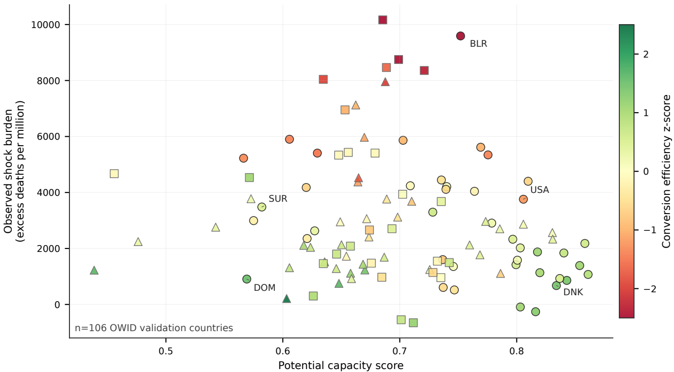
Capacity and observed burden separate under pandemic shock
