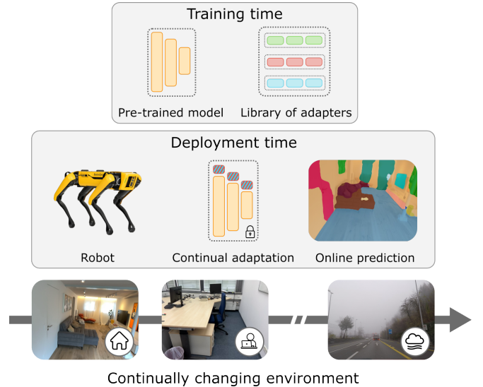
Fig. 1. The training-free continual test-time adaptation task considered in this paper.
