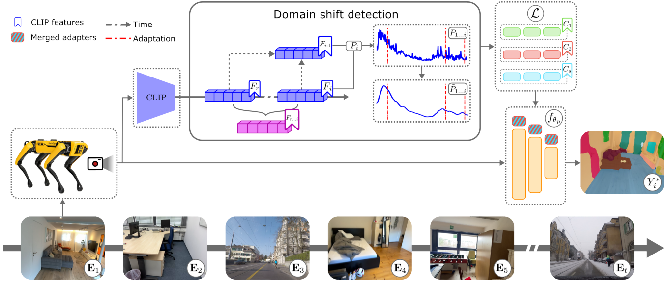
Fig. 2. General overview of the framework for training-free continual test-time adaptation, incorporating SemLA [8] and our domain shift detector.
