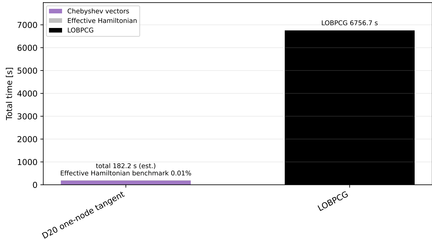
Total contraction time comparison (Chebyshev vectors + Effective Hamiltonian)
