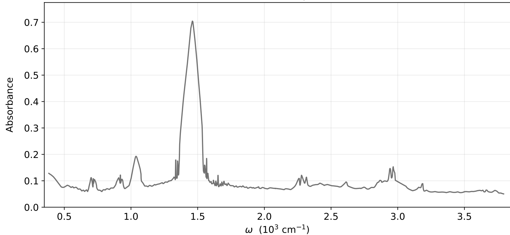
CH 3 CN infrared spectrum
