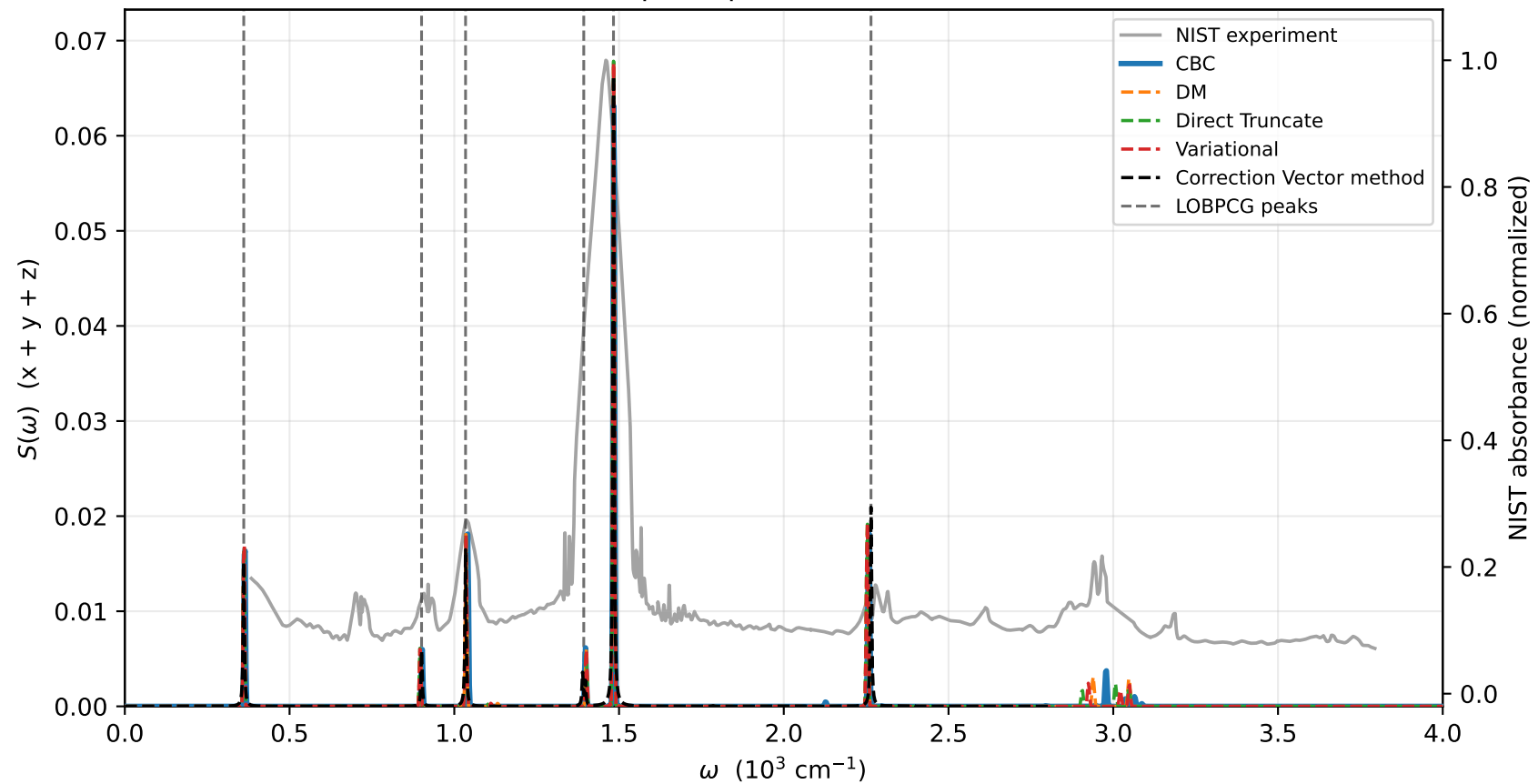
Dipole spectral function
