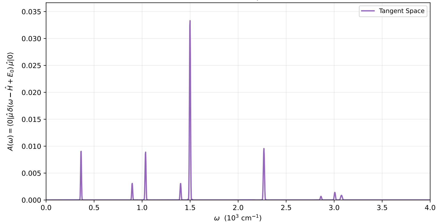
CH3CN infrared spectrum
