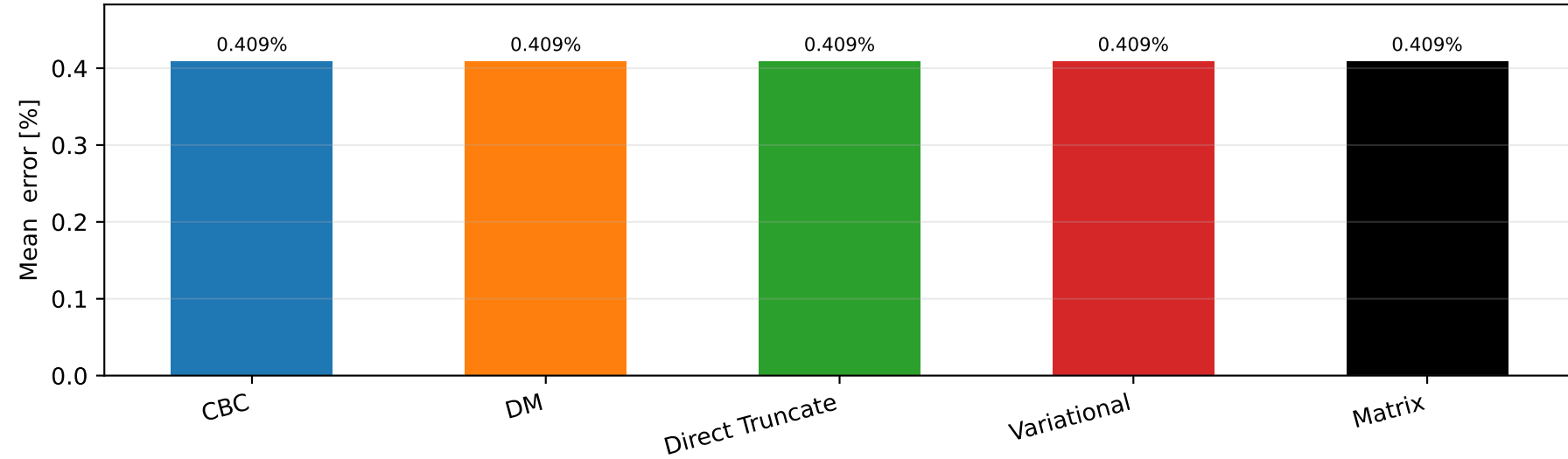
Mean H 2 O harmonic IR intensity error comparison
