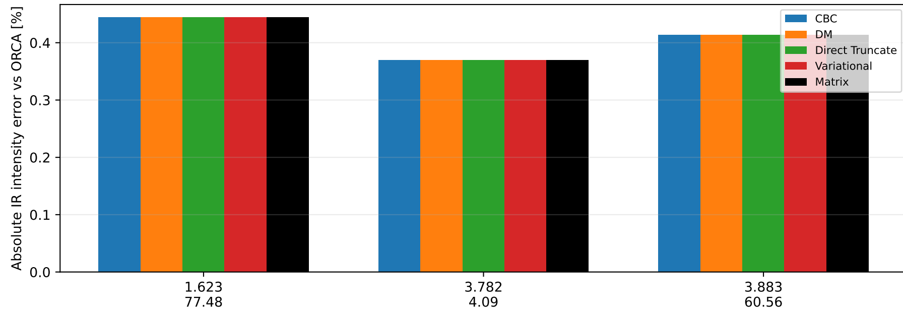
H 2 O harmonic IR intensity error comparison
