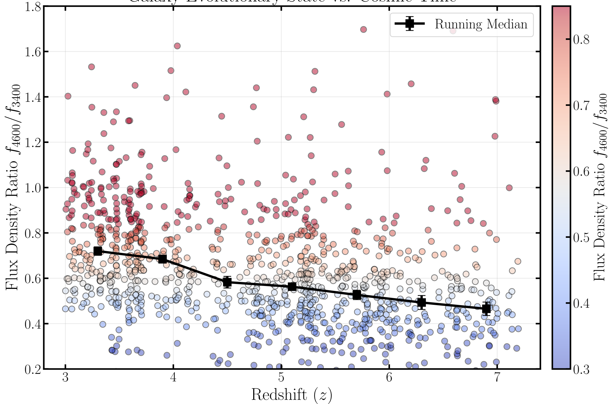
Galaxy Evolutionary State vs. Cosmic Time
