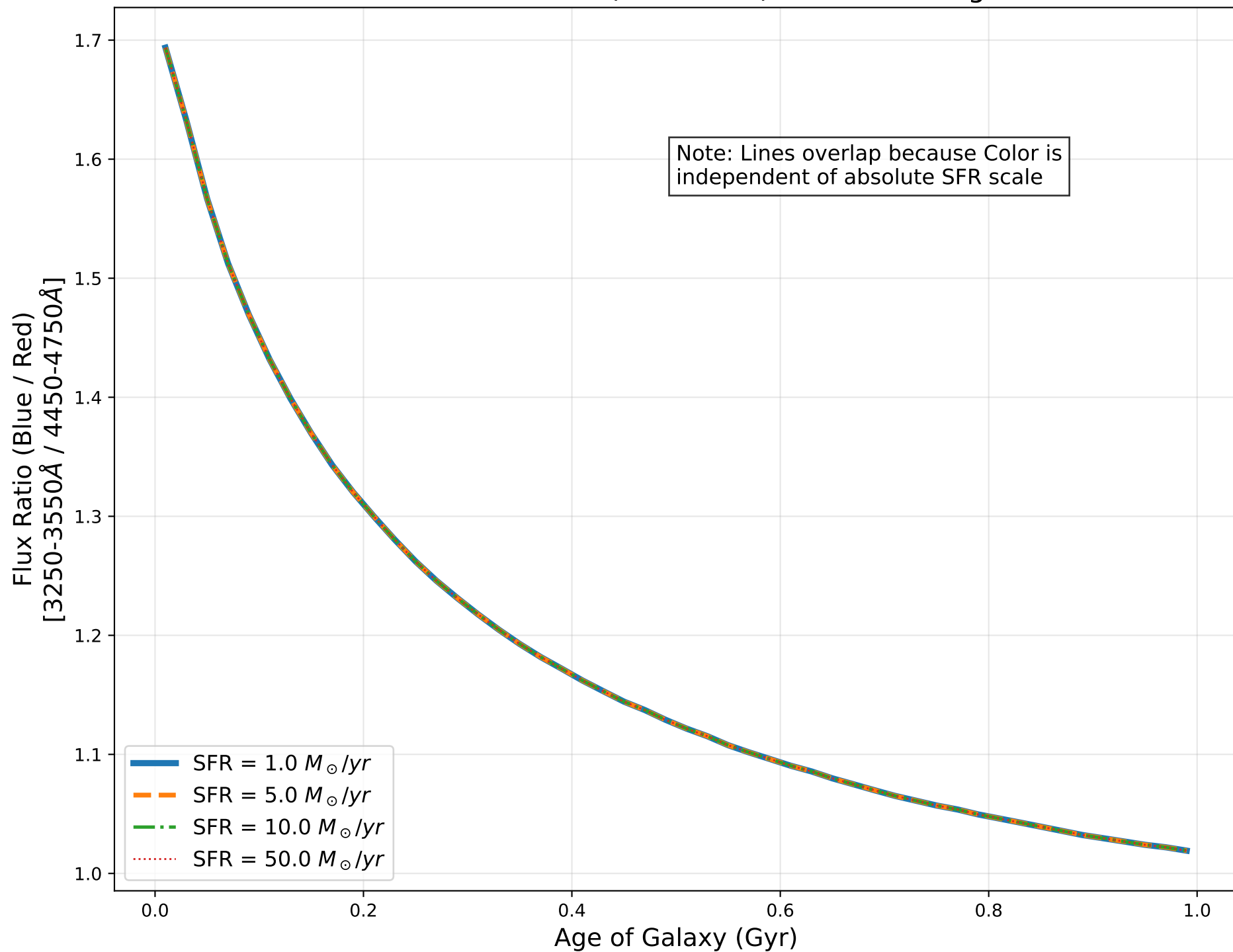
Evolution of Color (Flux Ratio) with Stellar Age
