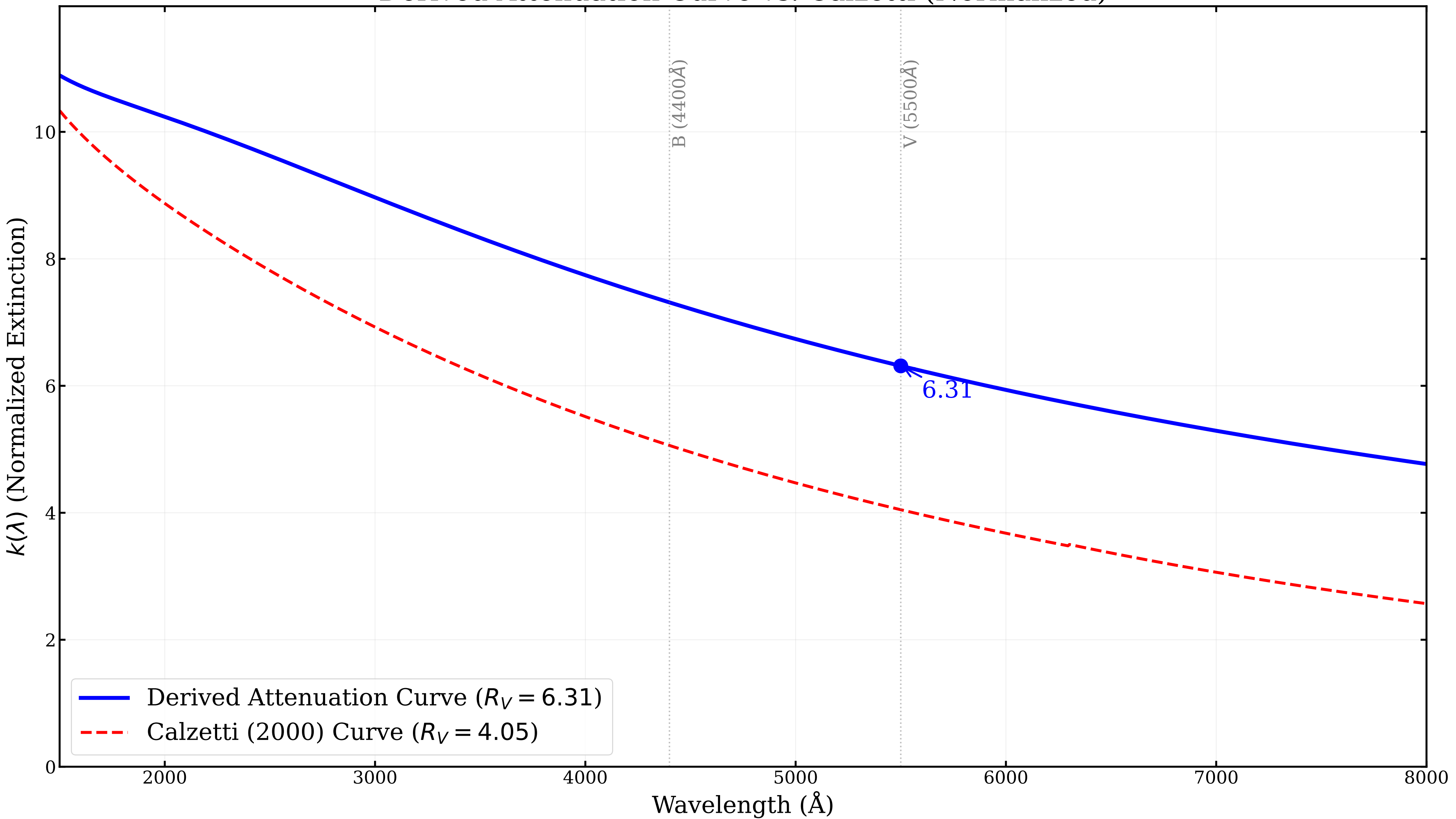
Derived Attenuation Curve vs. Calzetti (Normalized)
