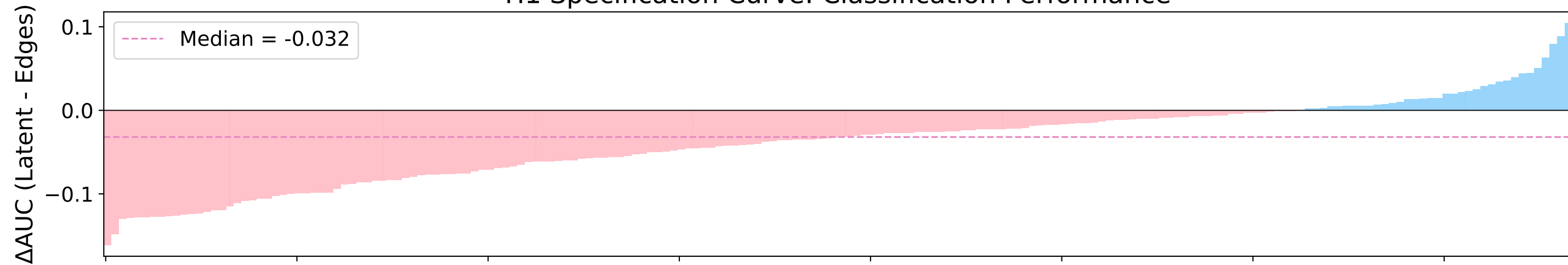
H1 Specification Curve: Classification Performance
