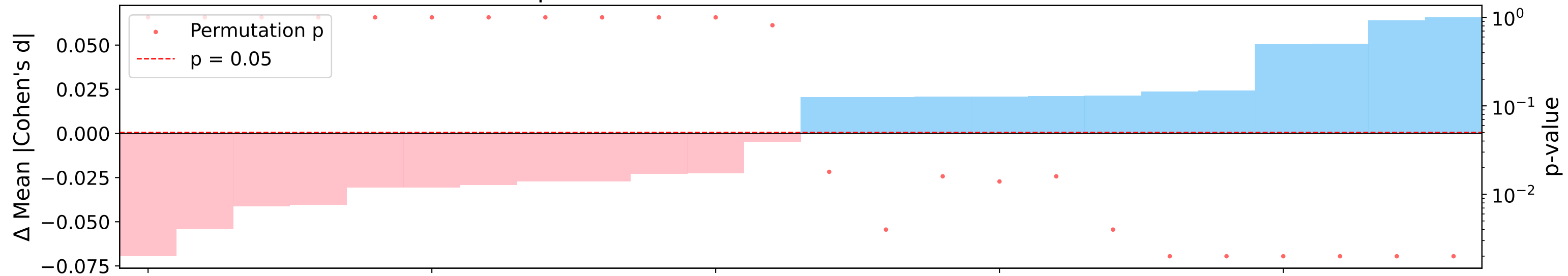
H2 Specification Curve: Between- vs. Within-Domain
