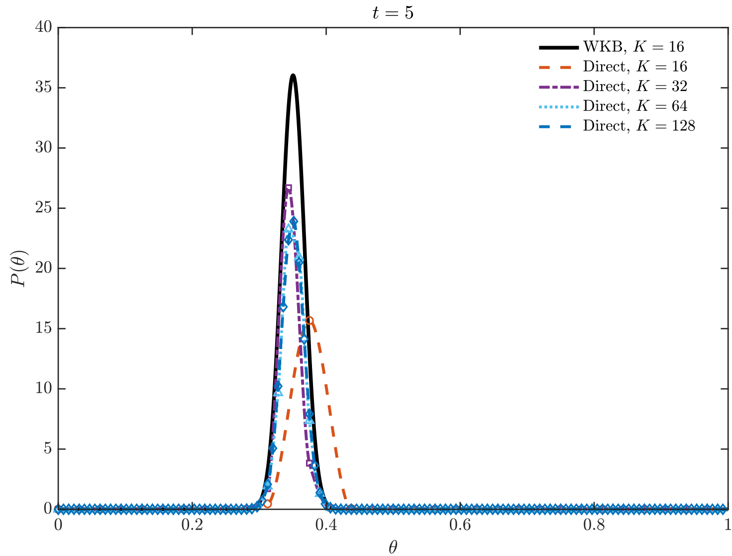
Trait marginal comparison, \varepsilon = 2.0e - 04
