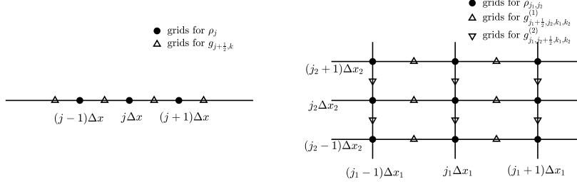
FIGURE 9. Illustration of the grids in \mathbf{x} -space for computing \rho(t, \mathbf{x}) and g(t, \mathbf{x}, \mathbf{v}) in 1D and 2D.
