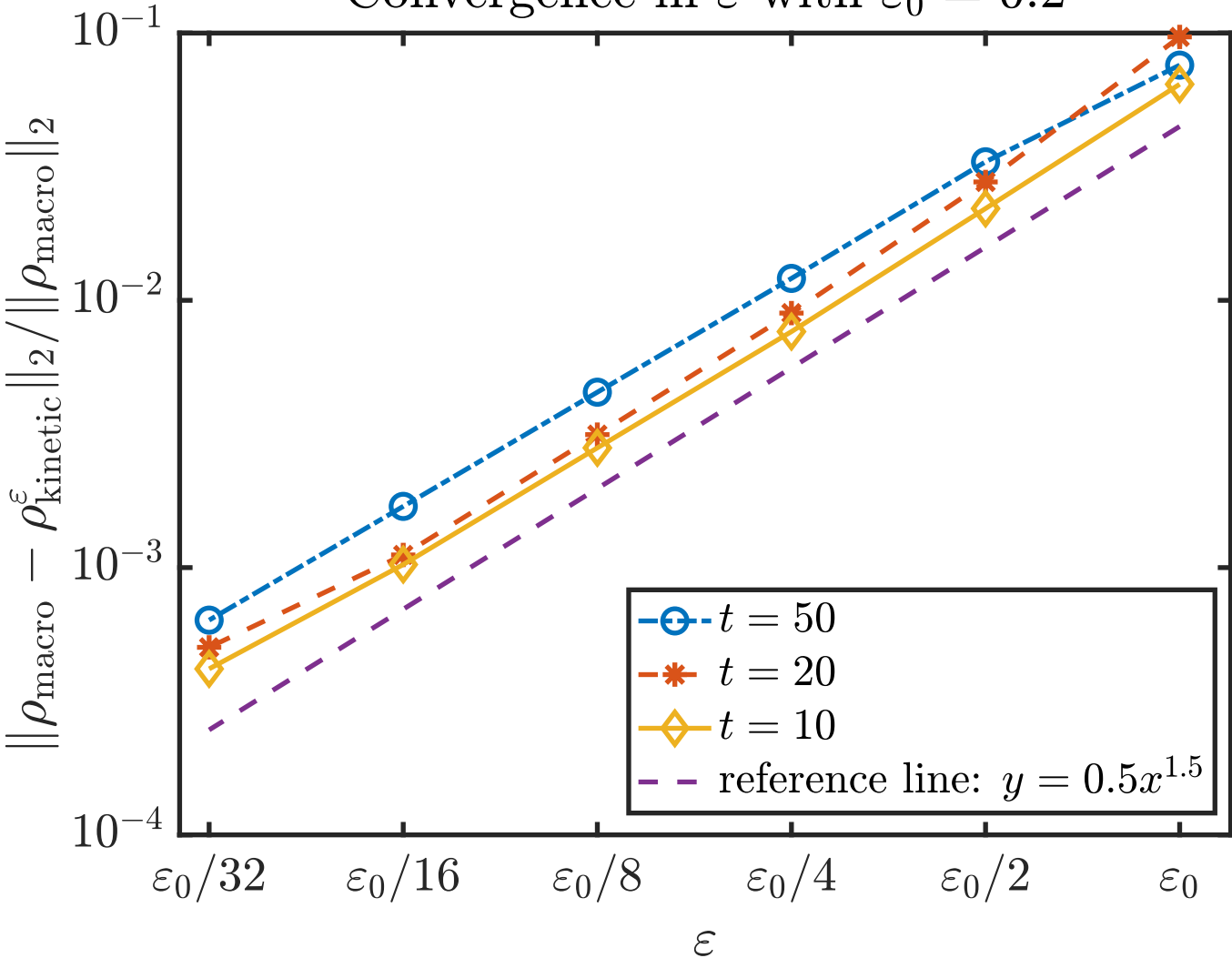
Convergence in \varepsilon with \varepsilon_0 = 0.2
