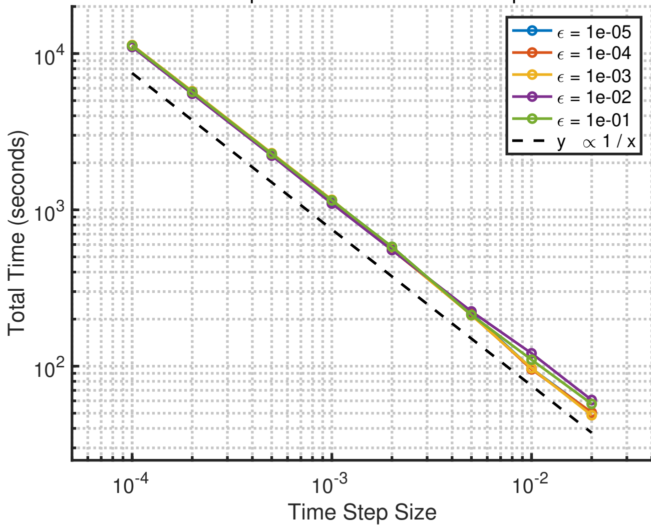
Total Computation Time vs. Time Step Size
