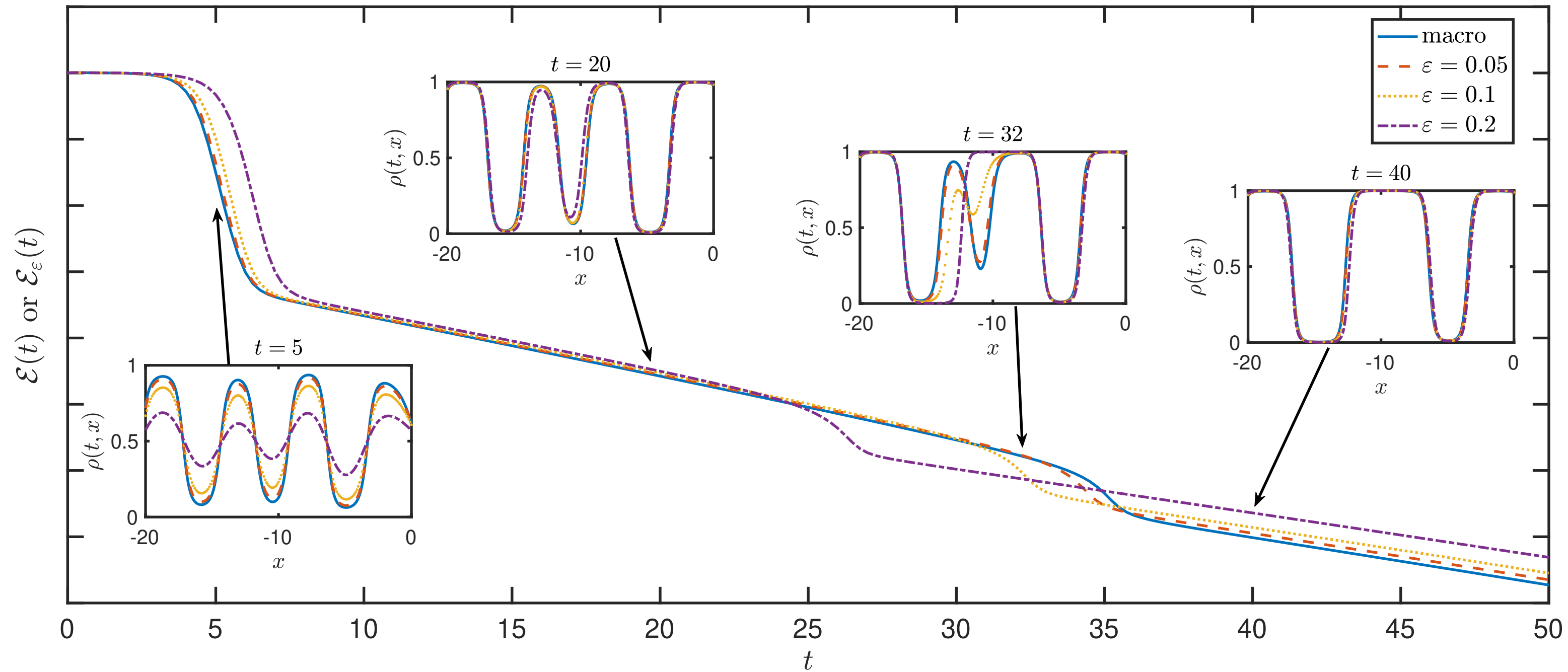
Evolution of energy \mathcal{E}(t) and \mathcal{E}_\varepsilon(t)
