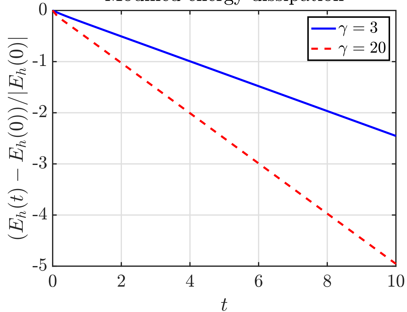
Modified energy dissipation
