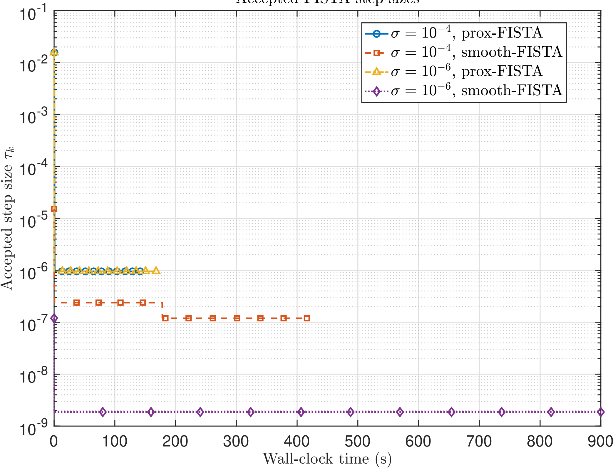
Accepted FISTA step sizes
