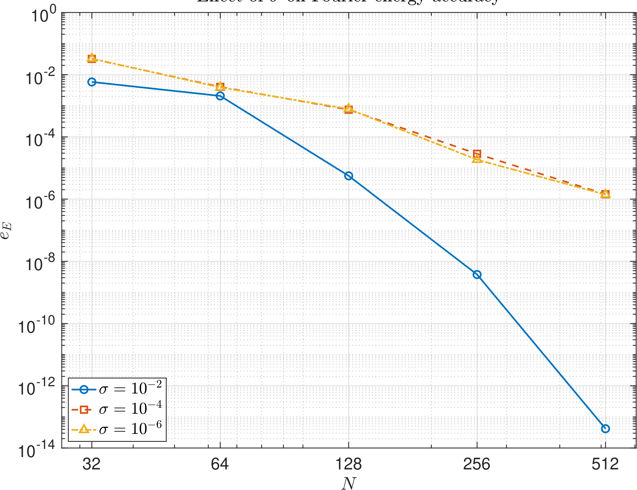
Effect of \sigma on Fourier energy accuracy
