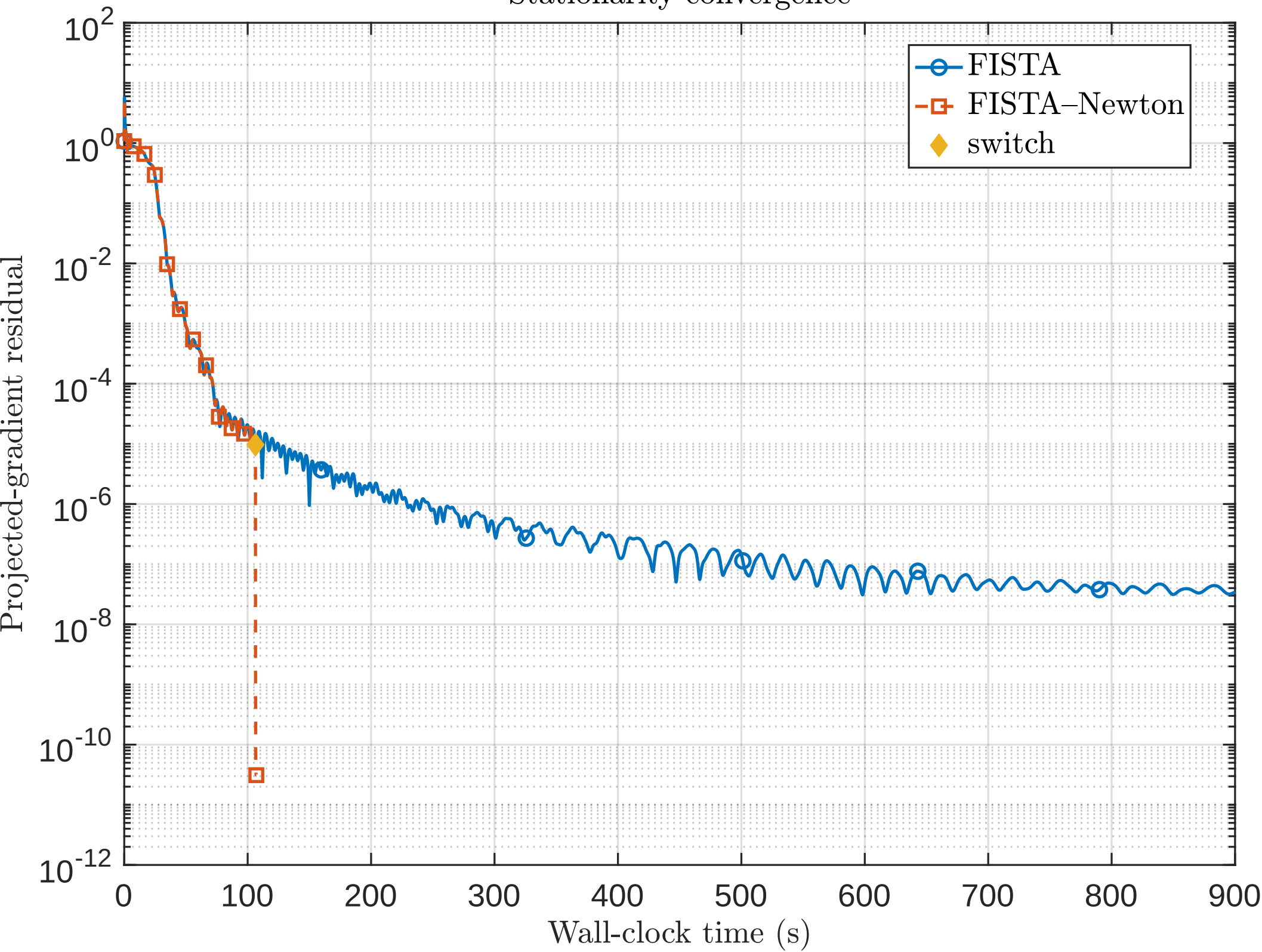
Stationarity convergence
