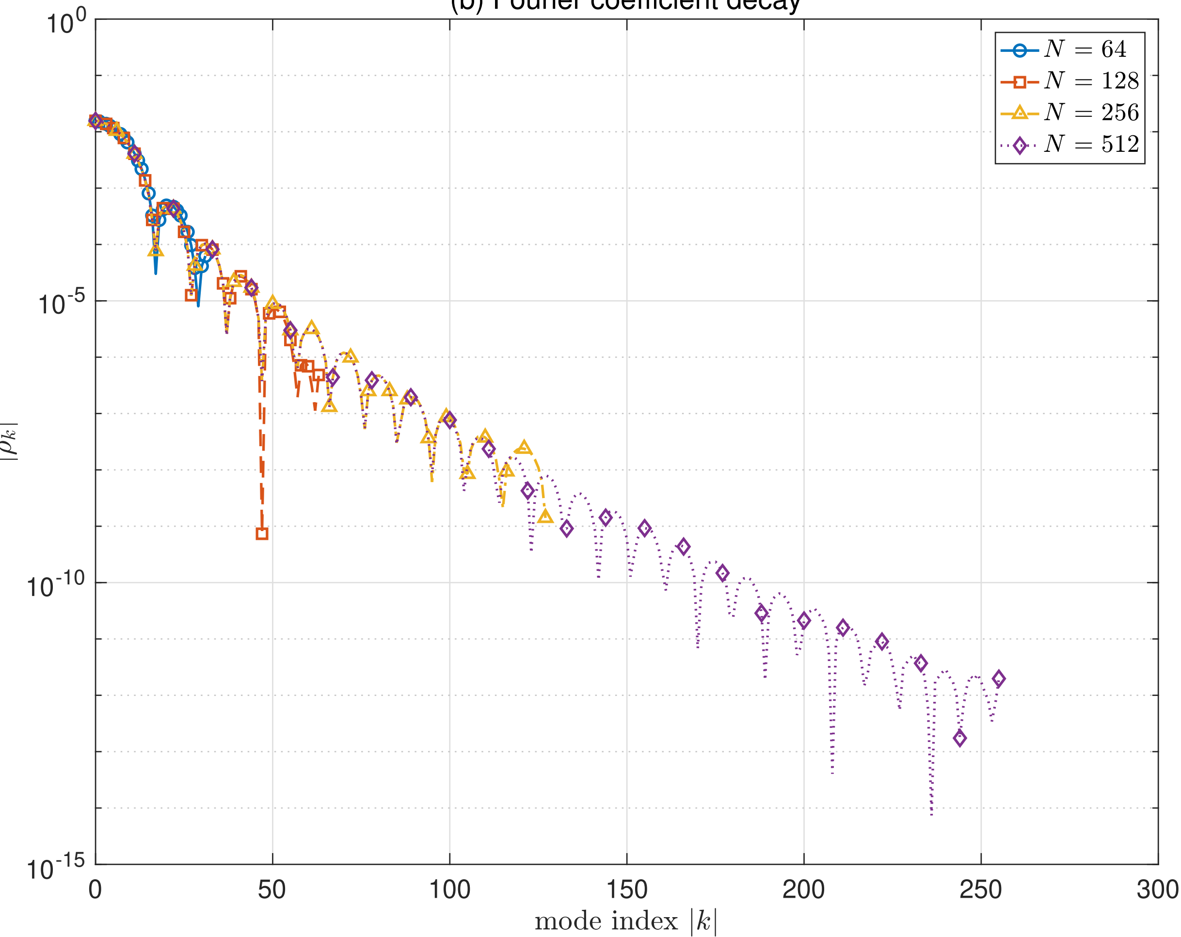
(b) Fourier coefficient decay
