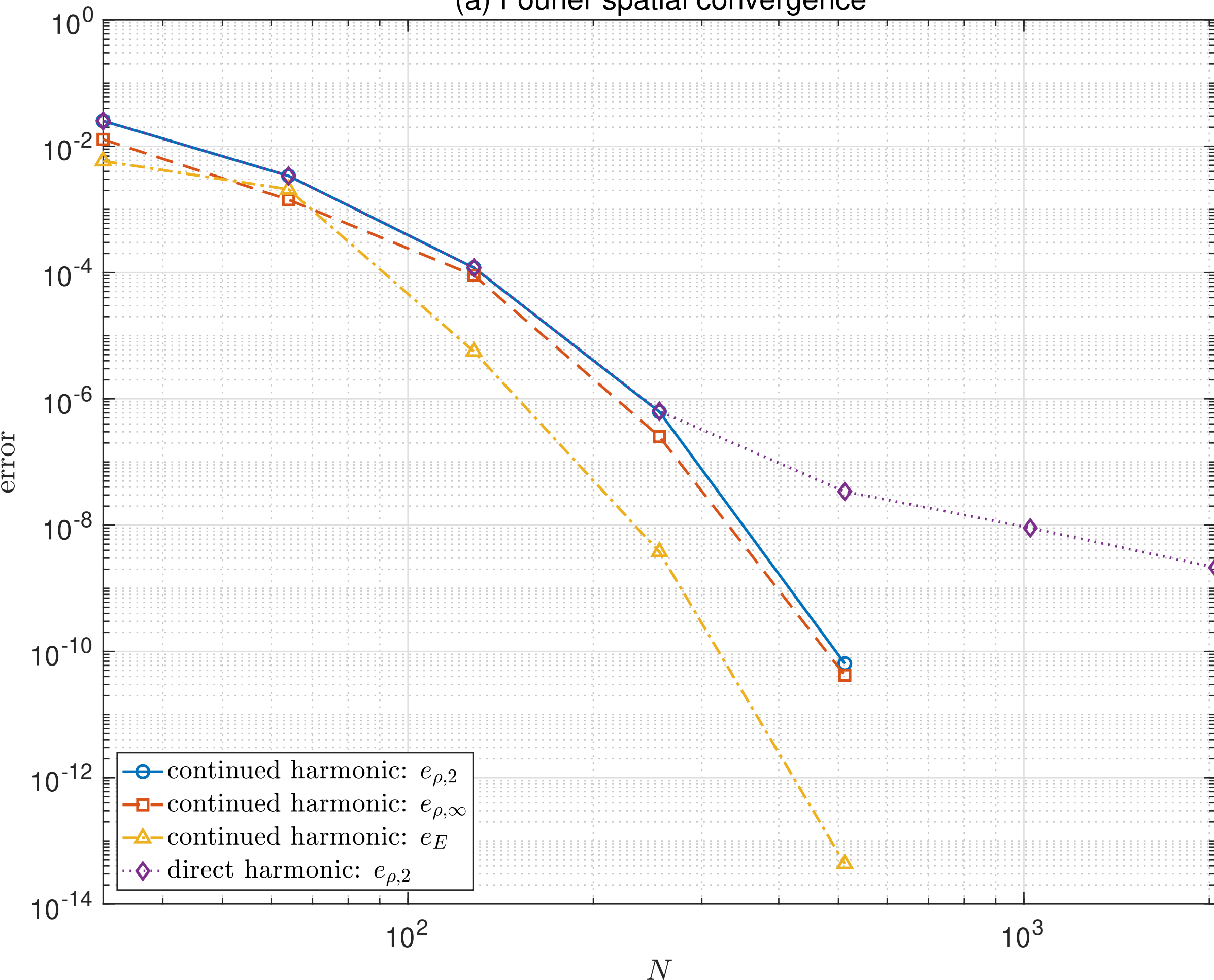
(a) Fourier spatial convergence
