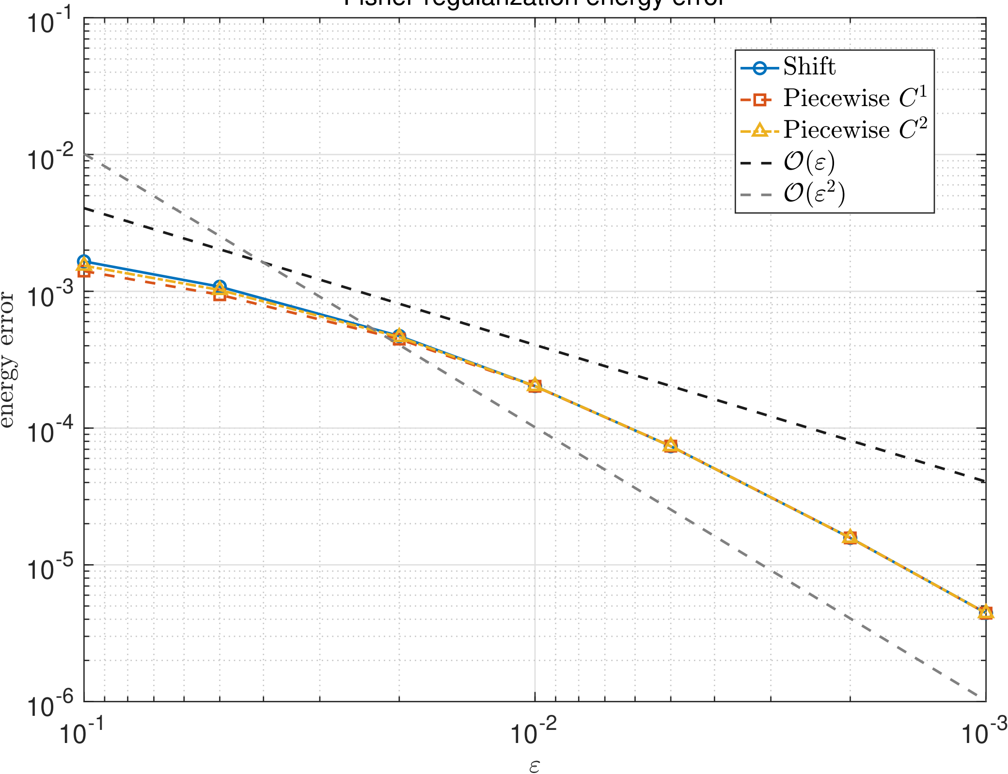
Fisher-regularization energy error
