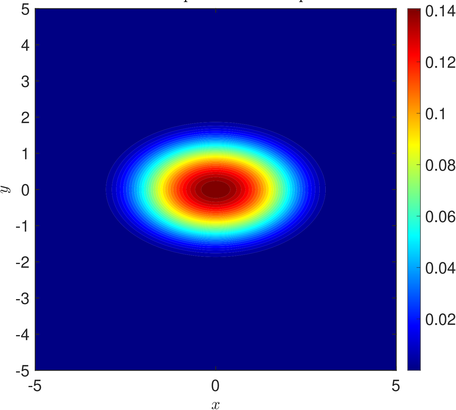
Anisotropic harmonic trap
