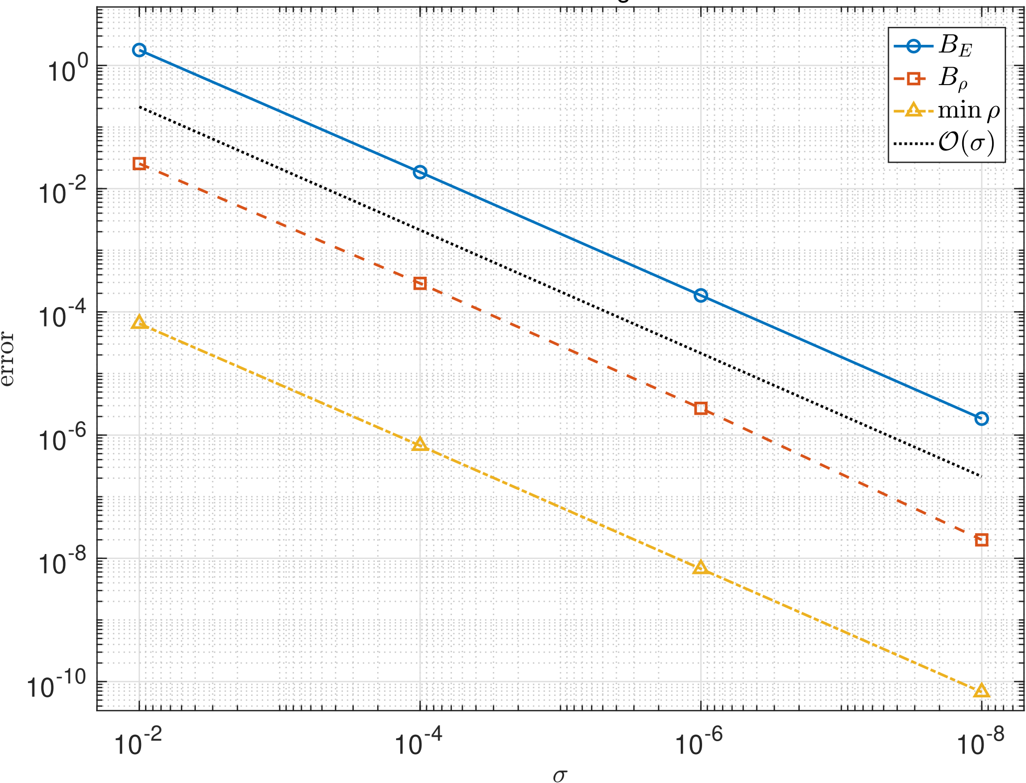
Potential-smoothing effects
