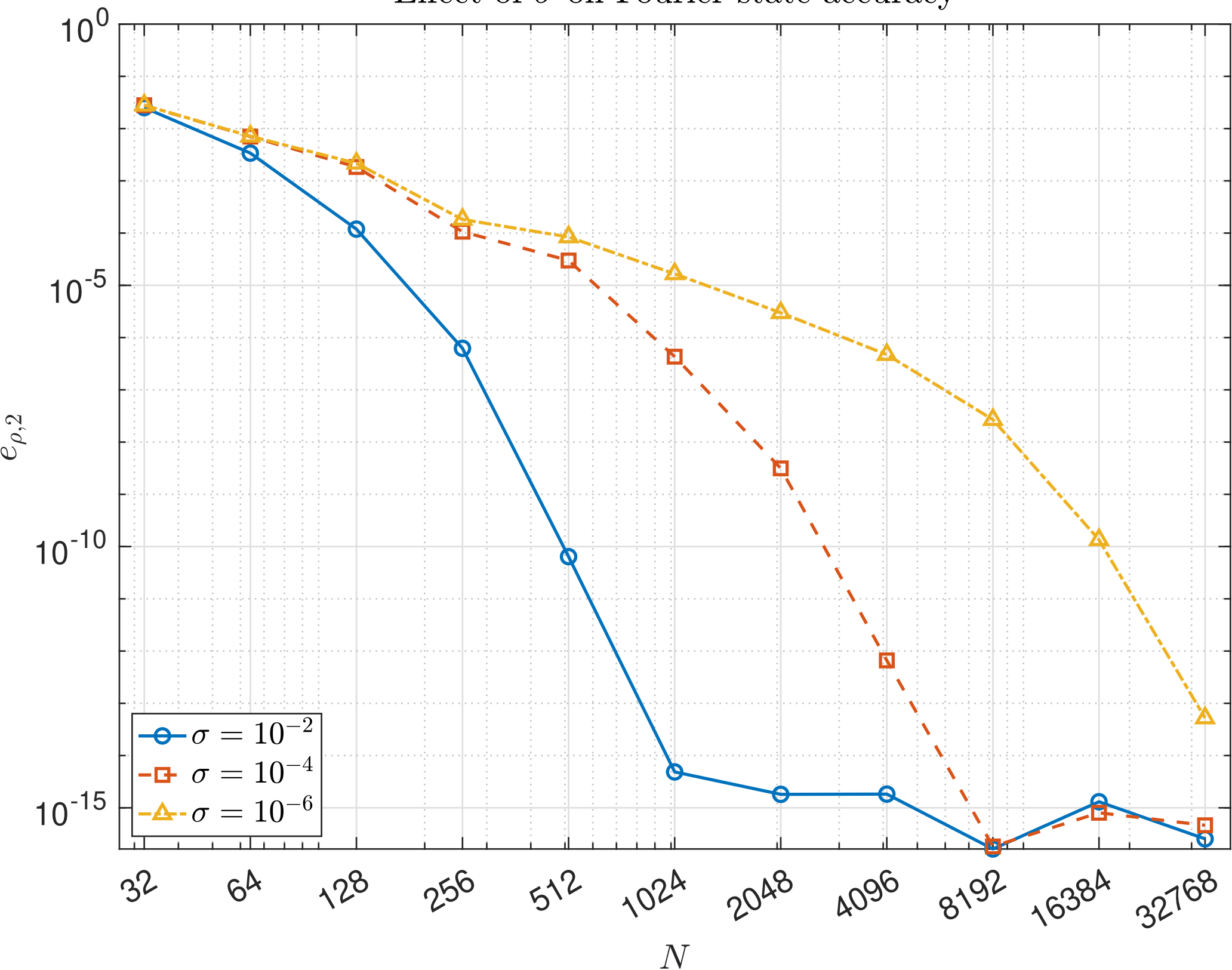
Effect of \sigma on Fourier state accuracy
