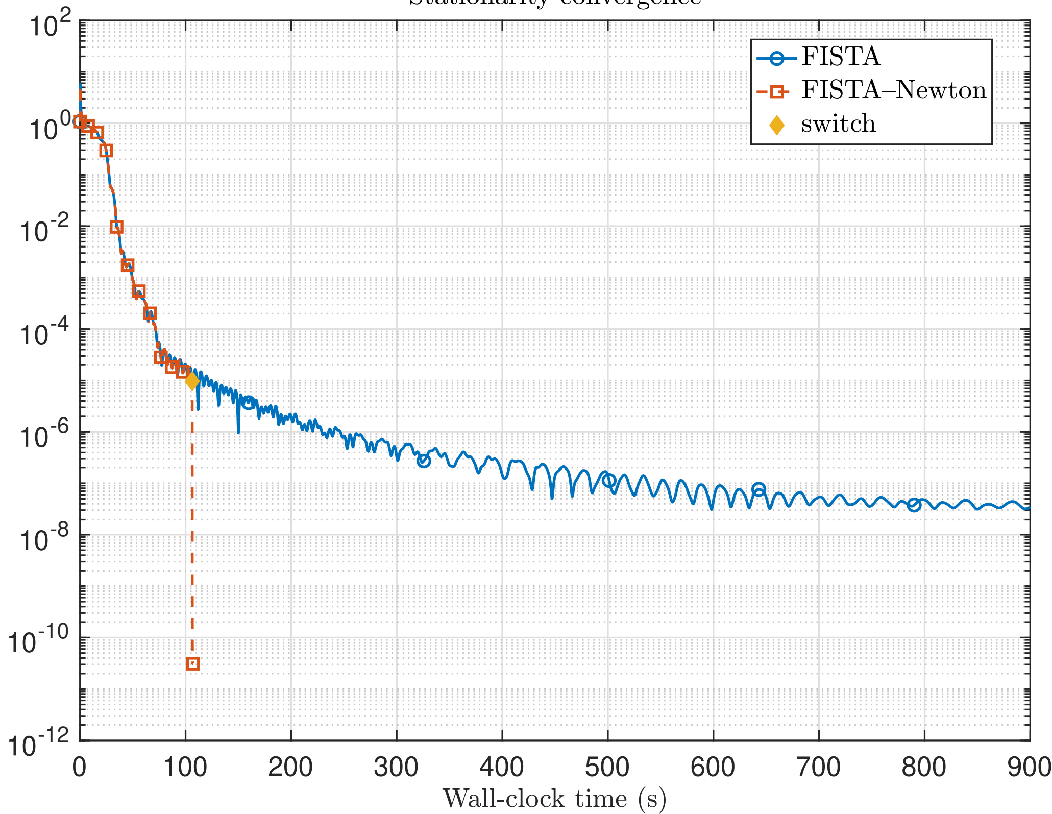
Stationarity convergence
