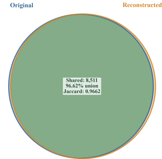
Protein Group quantified set
