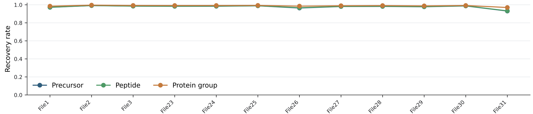
DIA-NN recovery by file
