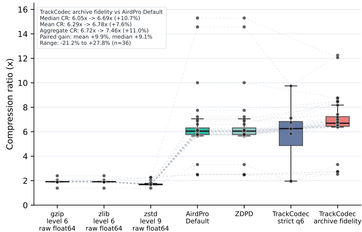
MS1 compression ratio distribution
