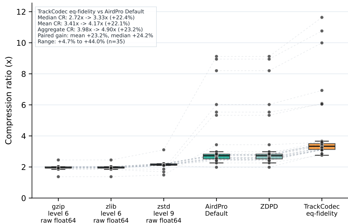
MS2 compression ratio distribution
