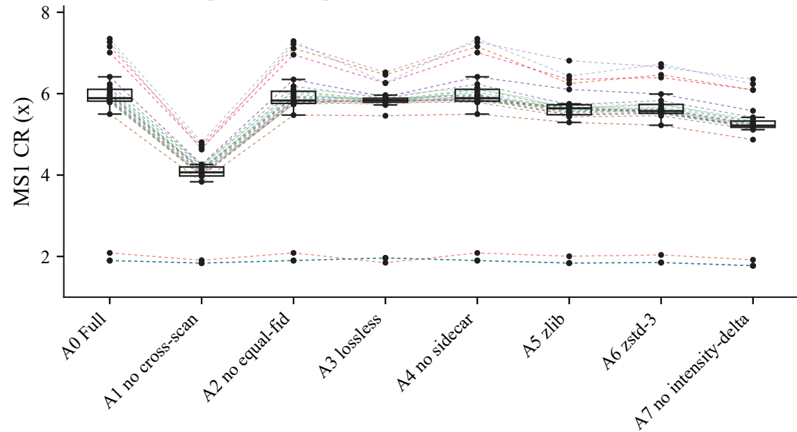
MS1 ablation: per-file compression ratio (n=30)
