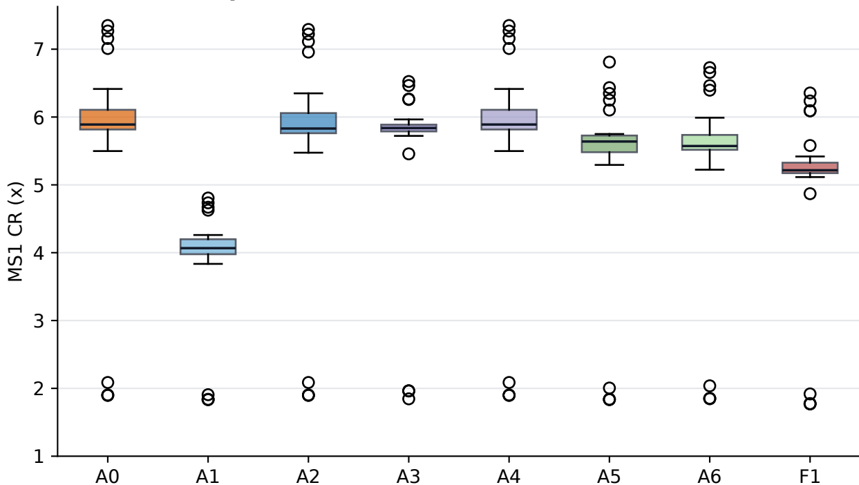
MS1 ablation per-file distribution
