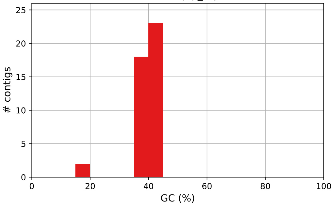
SRR13577846.asm.bp.p_ctg GC content
