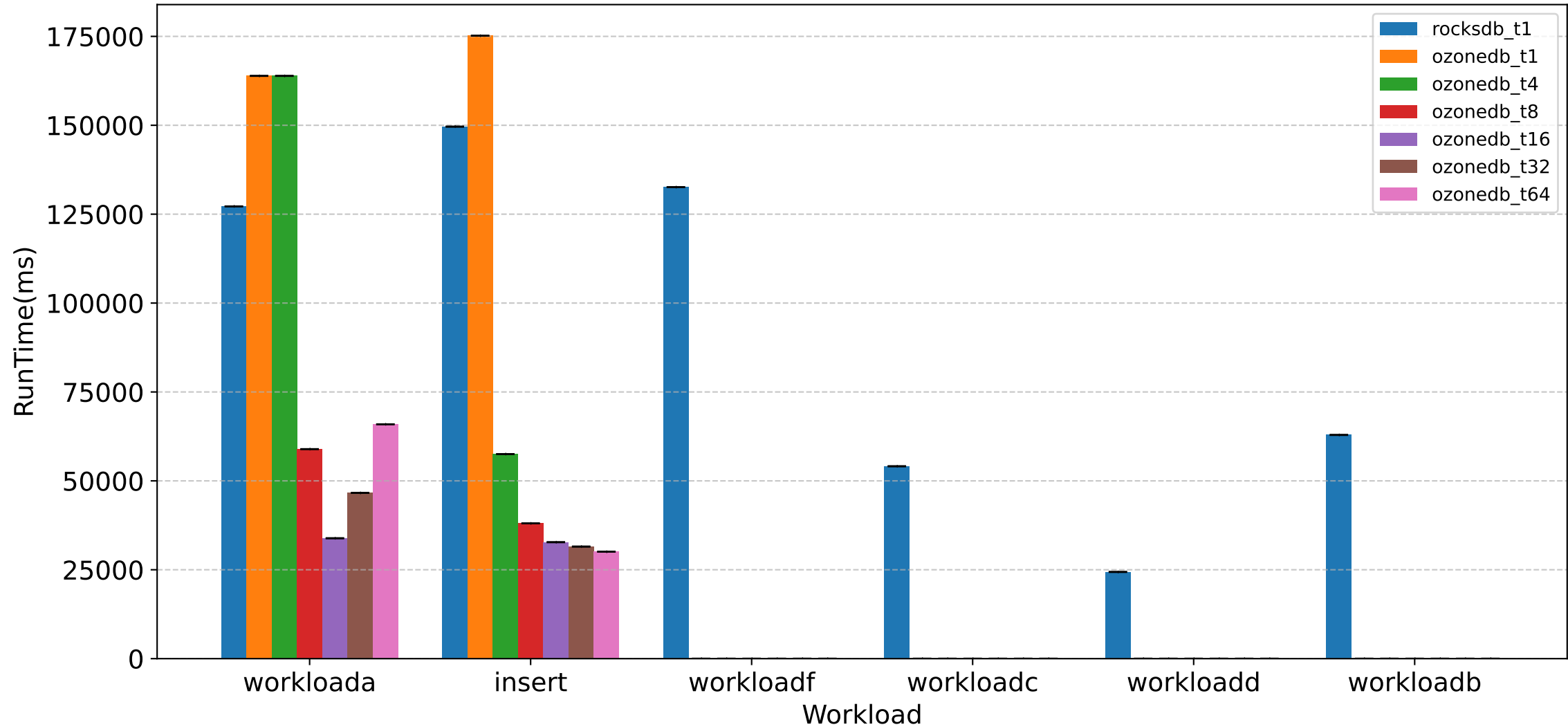
RunTime(ms) Comparison
