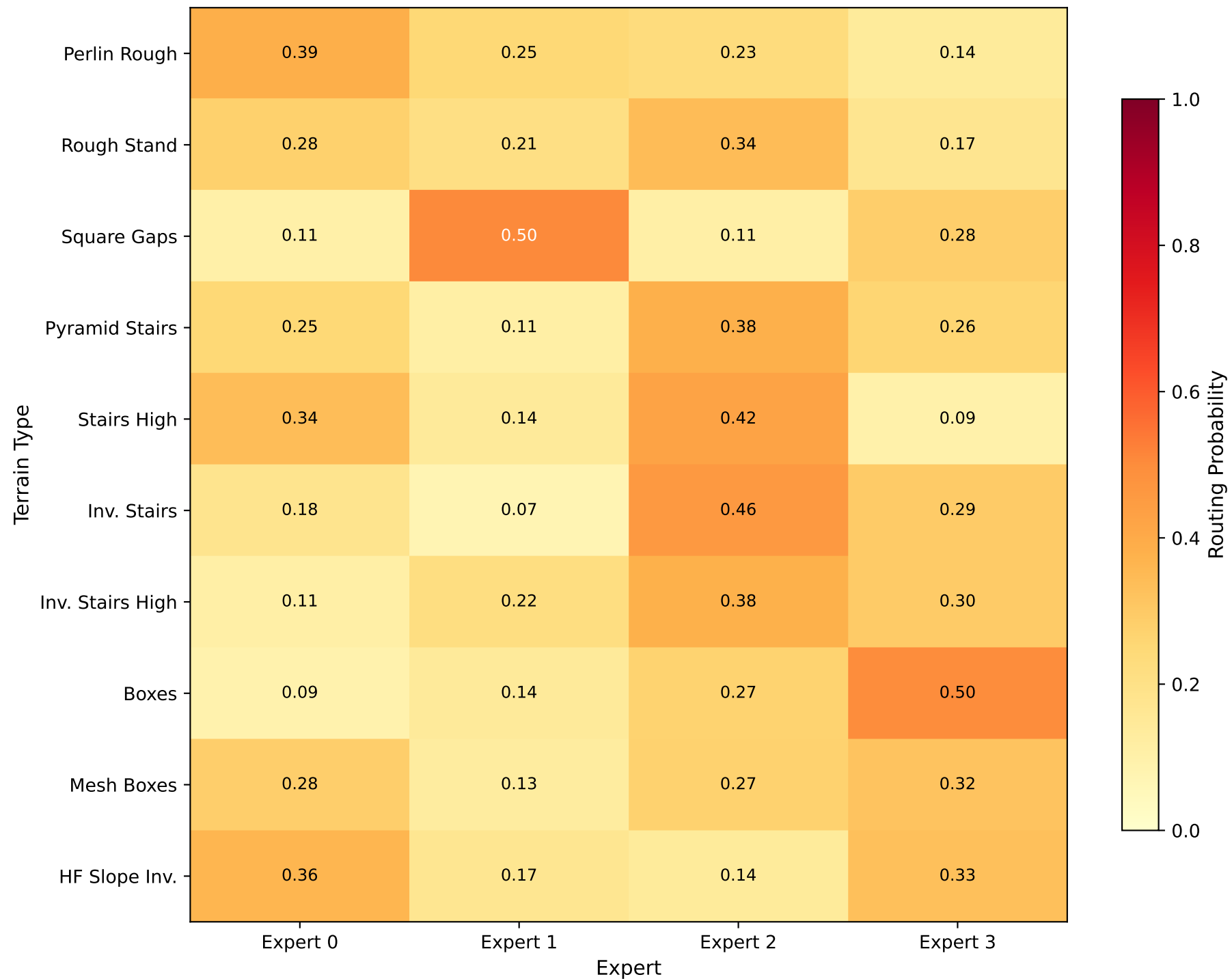
Expert Routing Distribution Across Terrain Types
