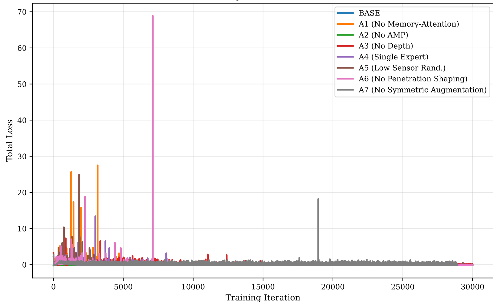
Total Loss vs Training Iteration for Ablation Variants
