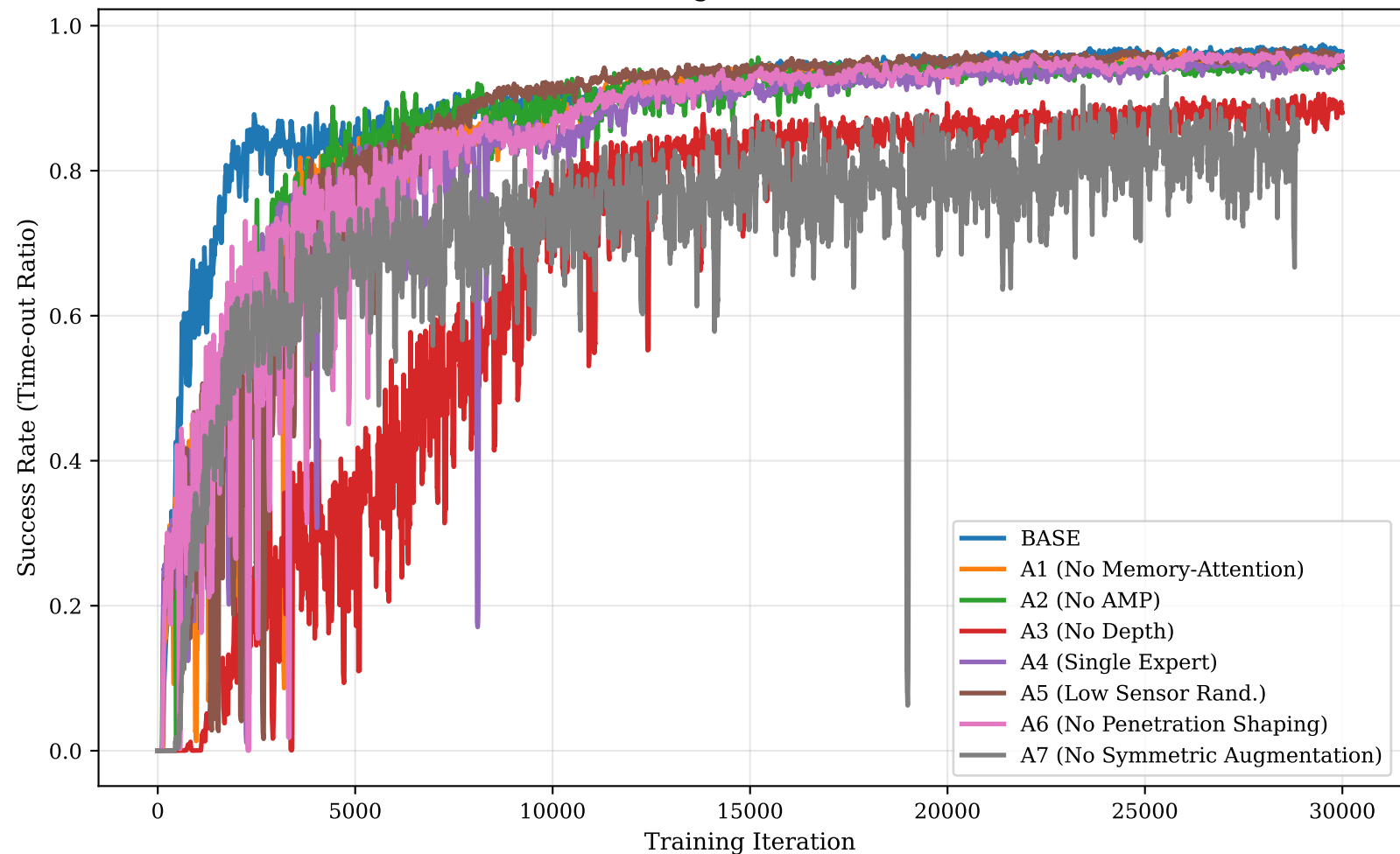
Success Rate vs Training Iteration for Ablation Variants
