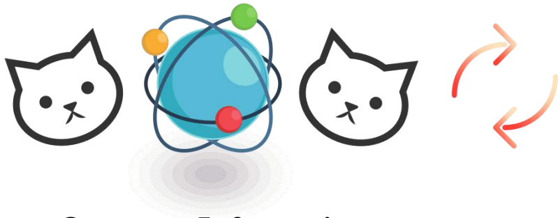
Quantum Information
