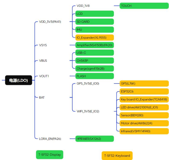
Power Control Diagram
