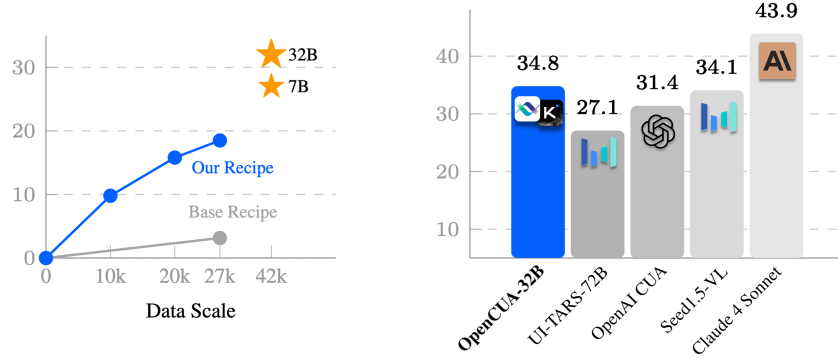
Figure 1: Left: OpenCUA recipe helps performance scaling with data size and model size. Right: OpenCUA-32B outperforms current open-source models on on OSWorld-Verified [43] and is comparable with OpenAI CUA (GPT-4o based) [28].
