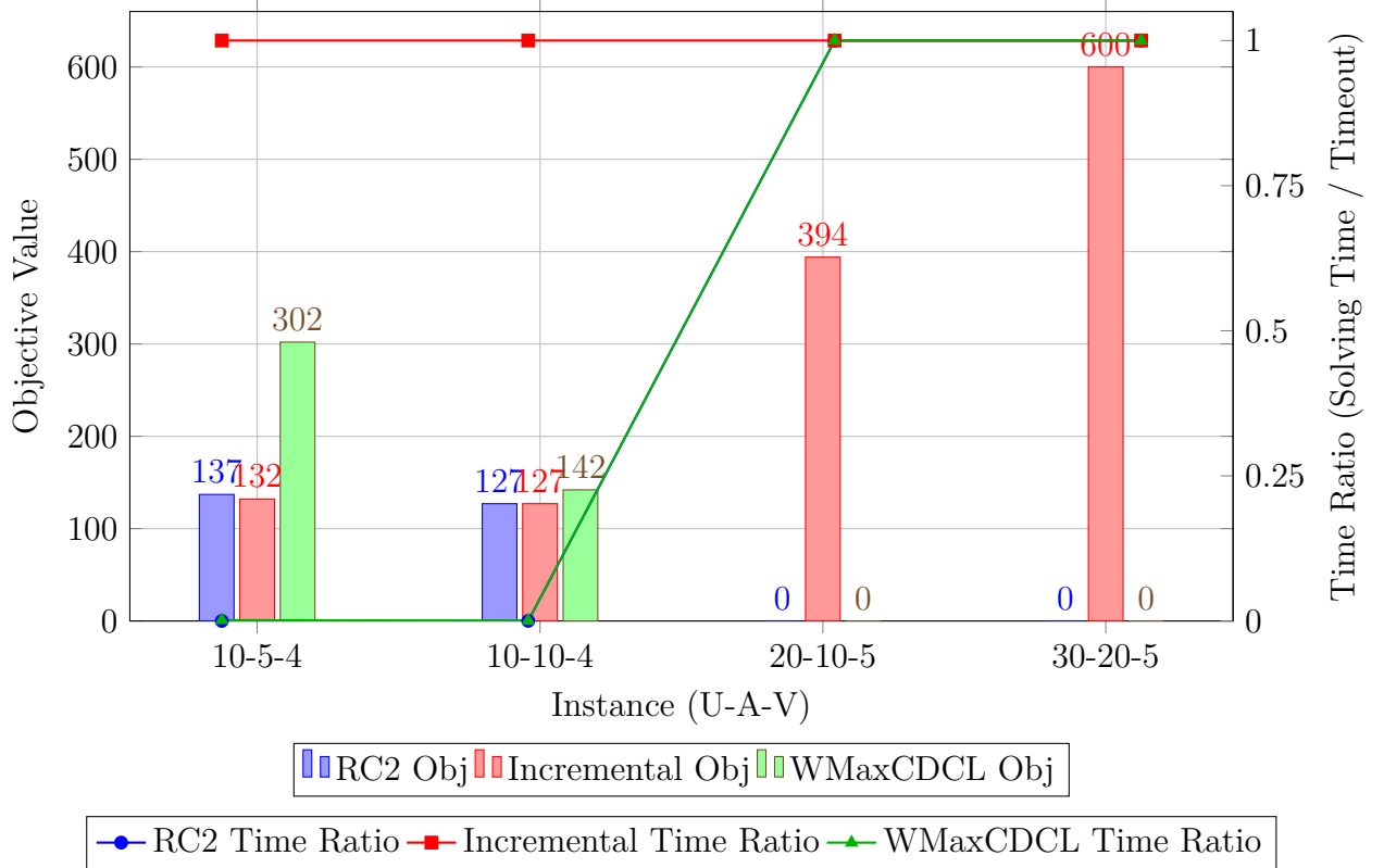
Figure 1: Comparison of HCORAP solvers: objective values (bars) and normalized solving times (lines). A ratio of 1 indicates that the solver reached the time limit.
