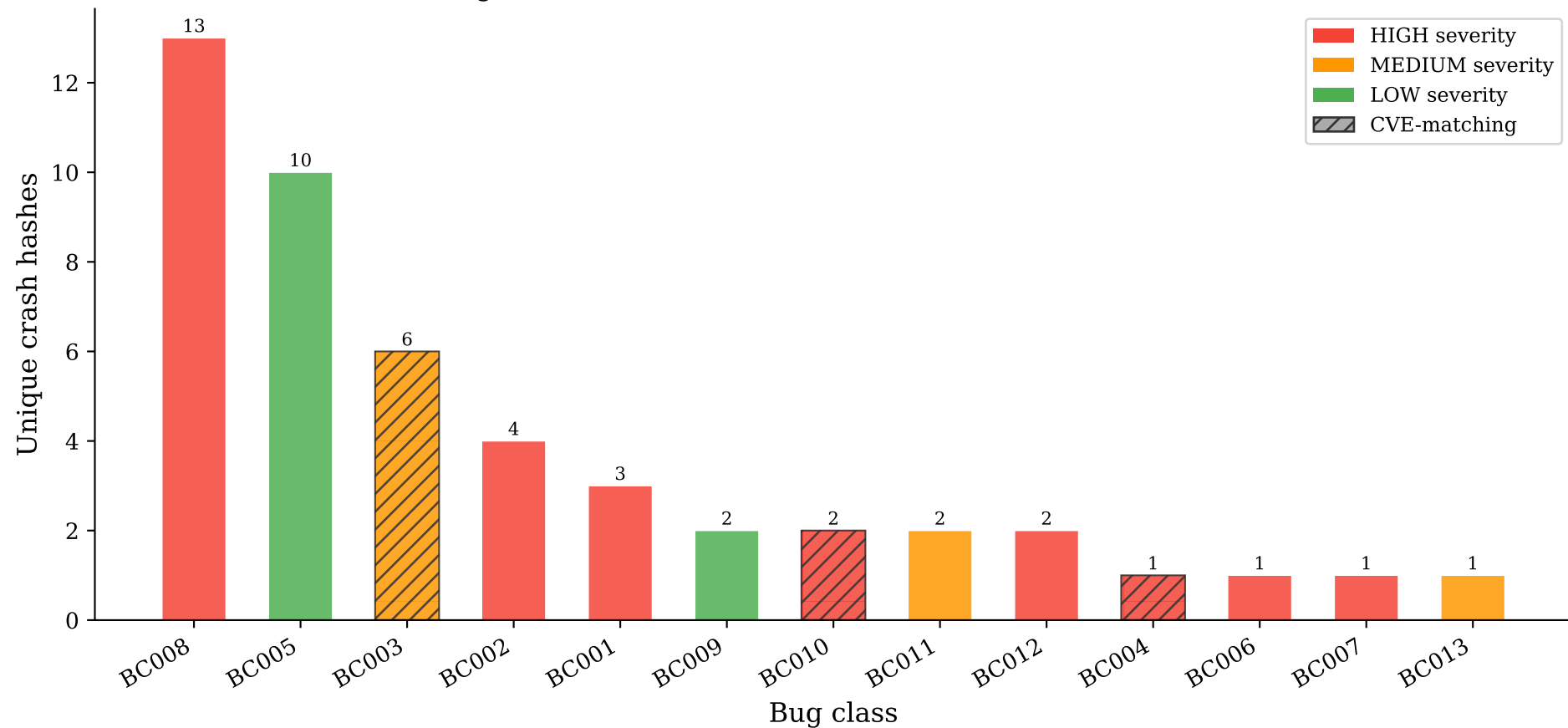
Bug Class Breakdown - DBMS-Nautilus (RQ2, 4 × 5 runs)
