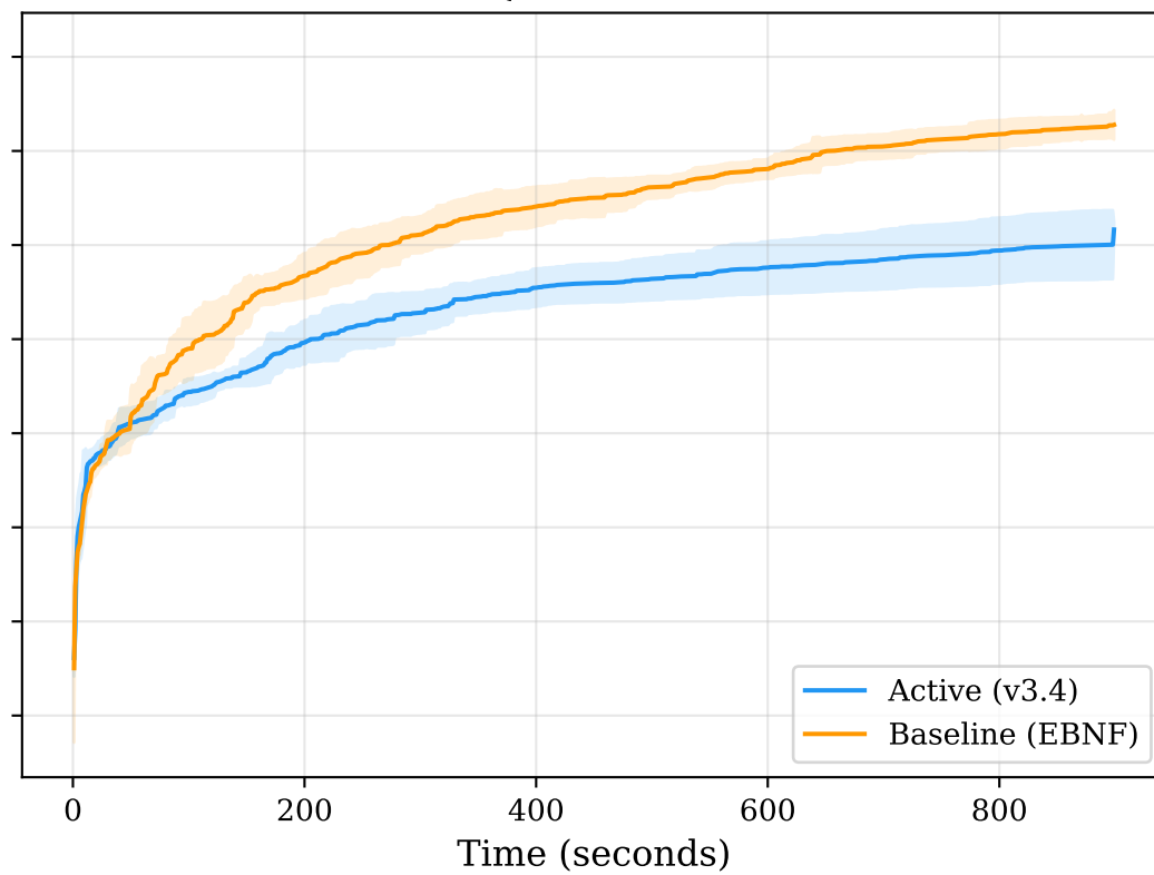
SQLite 3.32.2
