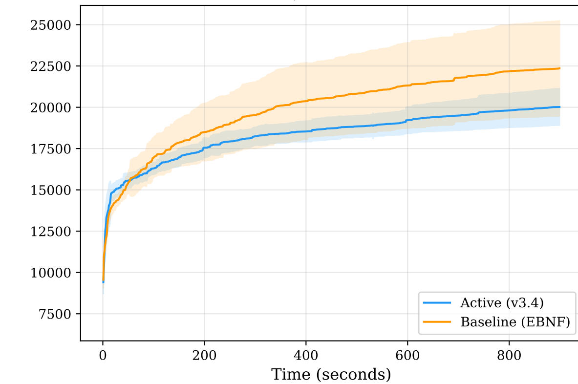
SQLite 3.32.0
